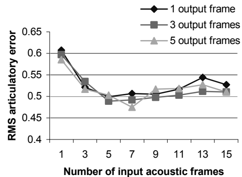
Figure 1. RMS articulatory error on artificial target as a function of network input and output window size.
