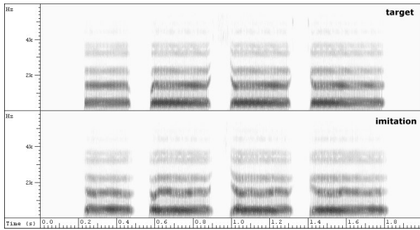
Figure 3. Top – artificial target phrase [əbədəgə], bottom – direct imitation using best inverse model.
