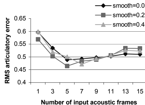
Figure 2. RMS articulatory error on artificial target phrase for a network with 30ms output window as a function of input window size and smoothing coefficient.
