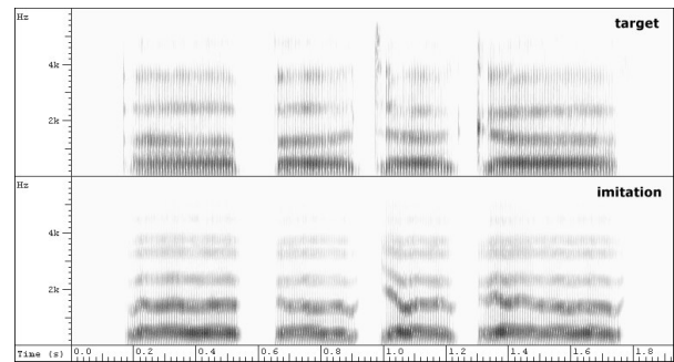
Figure 9. Natural target phrase and imitation using the combined method
