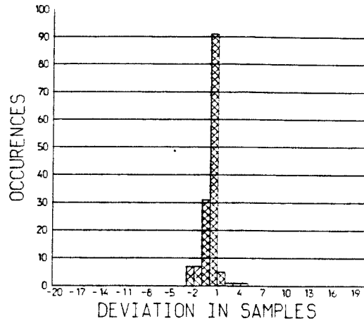
Figure 2: Jitter histogram for two Lx to Tx algorithms.
